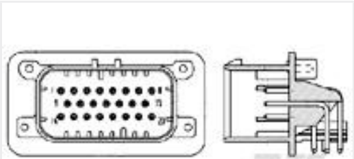
TE 产品编号1-776087-1 23POS,PIN DIA 1.3,HDR ASSY,90DEG, COD 1
