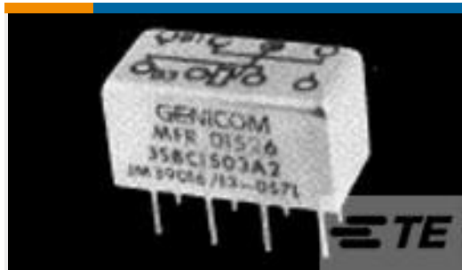
TE 产品编号1-1617073-3 3SBC2001A2 = M39016/13-056P
