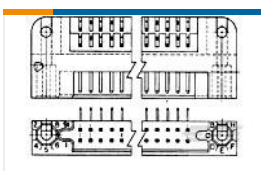
TE 产品编号531720-9 2 ROW BOX PIN 90 POS R/A
