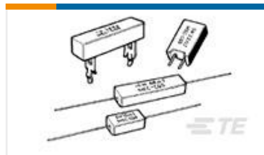
TE 产品编号1623781-9 SQMR10 10K 5% (METAL FILM)
