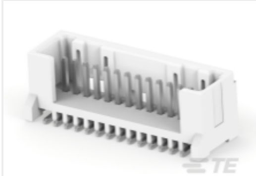
TE 产品编号1-2355091-4 MICRO CT CONN SINGLE ROW HDR ASSY(V)14p
