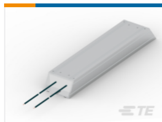
TE 产品编号2176465-6 HCH265 400W 82R 5% LEAD
