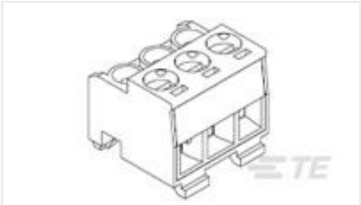
TE 产品编号1546173-2 5MM PLUG, 90/180, 2 POS, GREEN, SN
