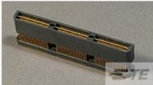
TE 产品编号1658017-3 MSB0.80PL19ASY120FL,-,10,-TY
