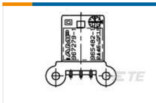
TE 产品编号967279-1 3pos MQS .63 header 90deg THR
