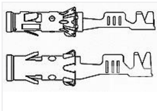
TE 产品编号962952-1 4MM SOCKET CONTACT
