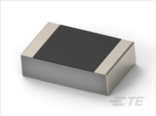
TE 产品编号5-2176452-5 CPF 0201 1K96 0.1% 25ppm 1K RL
