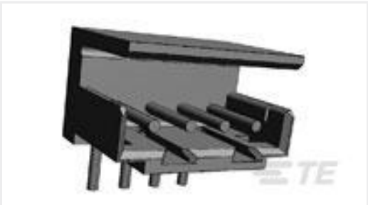
TE 产品编号292250-5 CT P/HDR BOX H ASSY 5P W/KINK
