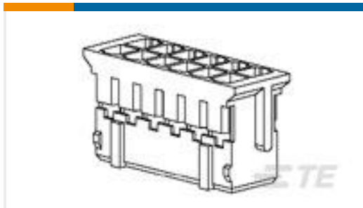
TE 产品编号1-1470107-2 2.0MM PITCH CRIMP HOUSING 12P
