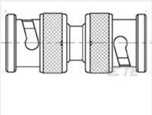
TE 产品编号1-1478043-0 BNC M TO BNC M ADAPTOR,STR,75 OHM,2G
