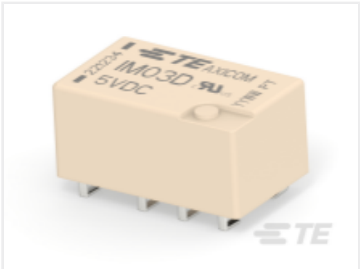
TE 产品编号 3-1462039-3 IM03DJR=IM RELAY 140mW 5V
