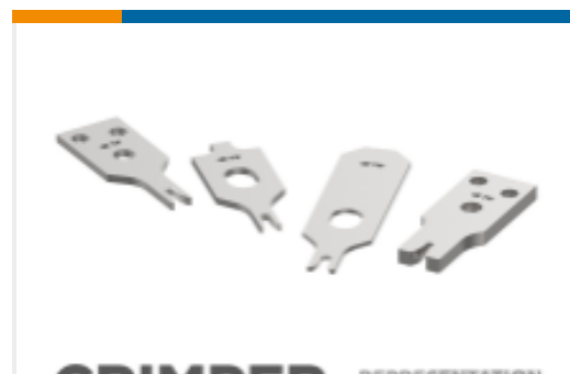
TE 产品编号6-1752057-0 CRIMPER, WIRE PREMIUM, STEPPED
