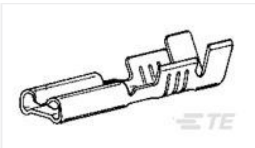
TE 产品编号140717-2 110 FASTON,REC.,22-18 AWG,PTBR
