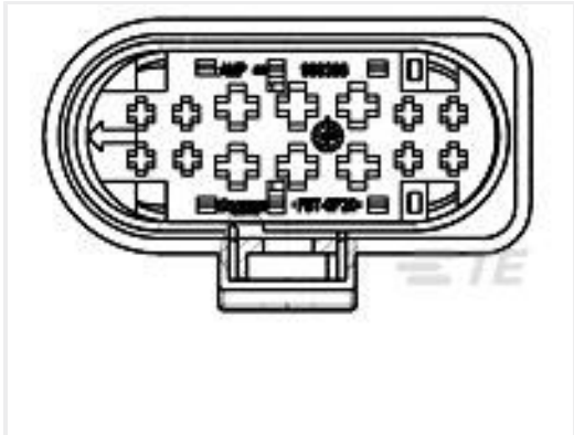
TE 产品编号1719105-2 14POS,JPT,REC. HSG
