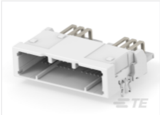
TE 产品编号2822546-1 0.5/1.5 38P CAP ASSY THR TYPE
