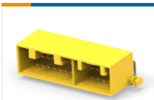
TE 产品编号1-5172491-7 PULSE LOCK CAP HSG ASSY 30P
