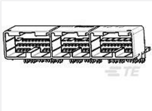
TE 产品编号1-1318751-2 025/090 80POS CAP ASSY H SELECTIVE-TIN
