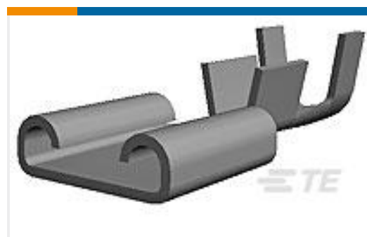
TE 产品编号170095-1 250 FASTON,REC.,22-18 AWG,TPPB
