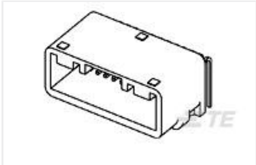
TE 产品编号1376357-8 025/090 26POS CAP ASSY H SELECTIVE-TIN
