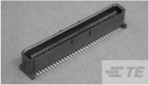
TE 产品编号2007009-2 84 1.0MM FH RCPT W/ COVER 8,9,10H
