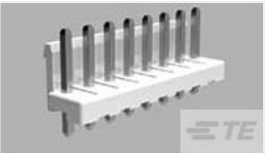
TE 产品编号1-1123723-7 3.96 EP HDR ASSY 7P(NATURAL)
