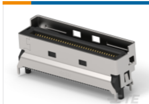
TE 产品编号2379397-6 MCIO INTERGRATED CONN, V/T,8X, SMT TYPE
