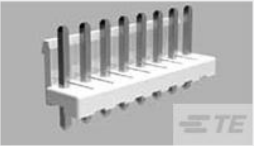
TE 产品编号4-1123723-5 3.96 EP HDR ASSY 5P(RED)
