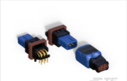
TE 产品编号YD369-B99-NS400000 369 9 WAY PANEL MNT REC, 90 PCB GOLD,SKT
