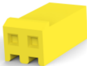
TE 产品编号644267-2 SL156 HSG (YELLOW)
