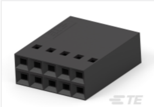
TE 产品编号 104482-4 10 SHORT PT RCPT HSG DR .100CL
