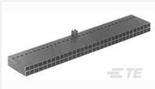
TE 产品编号1-104483-1 10 SHORT PT RCPT HSG DR .100CL
