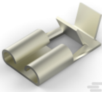
TE 产品编号1217972-2 250 FASTON, FLAG, REC., 18-14 AWG, NPST
