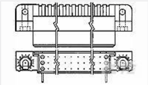
TE 产品编号533268-8 HDI RECP ASSY 3 ROW 165 POS
