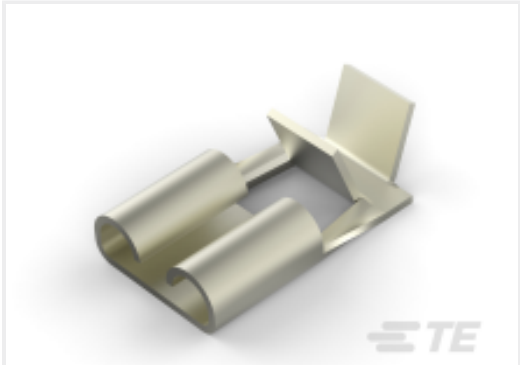
TE 产品编号1217972-2 250 FASTON, FLAG, REC., 18-14 AWG, NPST
