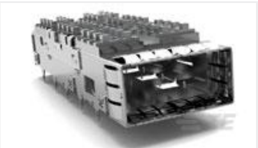
TE 产品编号2170395-1 Cage Assy PCI Hsink QSFP Behind Bezel
