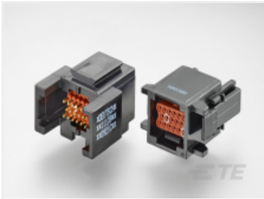
TE 产品编号ABC06N-16P IN-LINE PLUG
