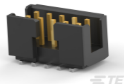
TE 产品编号1-2373376-0 10P,2MM,SHRD HDR,DRVT,SMD,0.1 AU,TB
