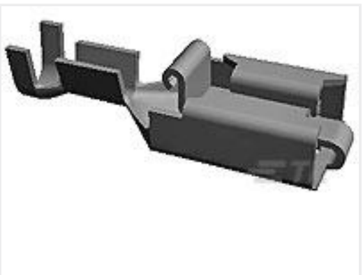
TE 产品编号154717-7 PL 250 REC TERMINAL 13-11 AWG PTPPB
