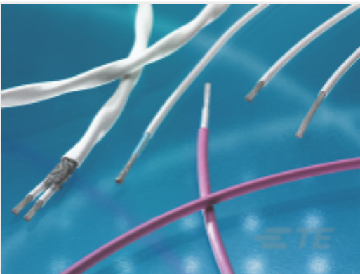
TE 产品编号CAT-55PC-TC-2T22 2 Core Twisted Pair Cable: Tin Coated Copper Cable, 22 AWG
