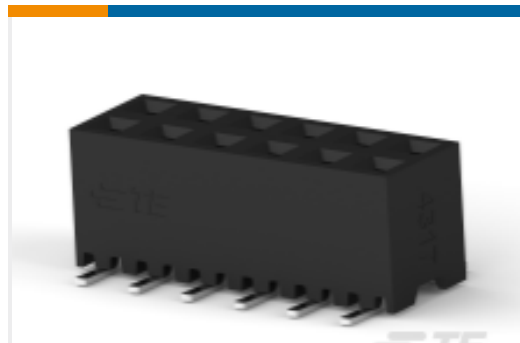
TE 产品编号1-2314846-4 14P,2MM,BB,REC,DRV,T,SMD,AU.76, TB,W/CP
