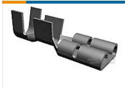
TE 产品编号280000-6 250 FASTON, REC., 24-17 AWG, TPBR
