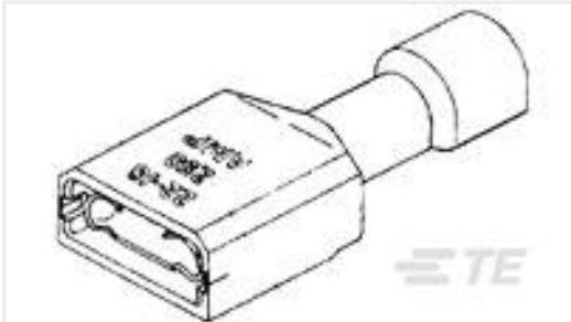
TE 产品编号3-350816-2 ULTRAFast 187 ASSY REC 16-14 TPBR LP
