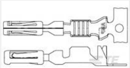
TE 产品编号770520-1 AMPSEAL,TERMINAL,TIN PLATE,16-20AWG WIRE
