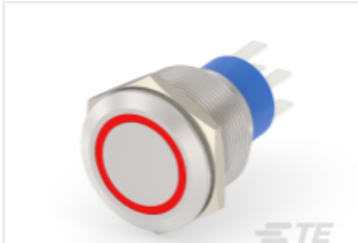
TE 产品编号6-2213772-7 AV22 DPL 3A MOVE RING LED RED 24V
