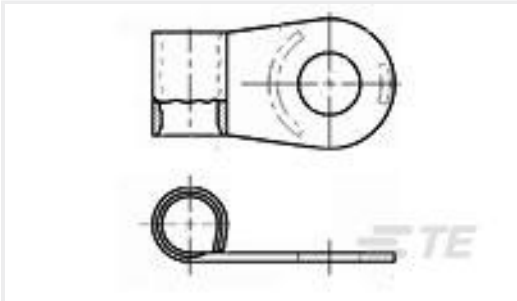
TE 产品编号36271 TERMINAL,SOLIS FLAG R 12-10 10
