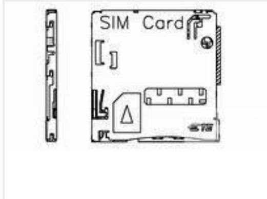
TE 产品编号2229333-2 PUSH-PUSH MICRO SIM CONNECTOR SMT-2 TYPE
