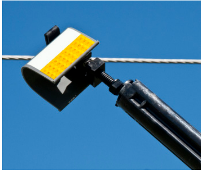
BCIC-AFD-01 Hot-stick Installation
