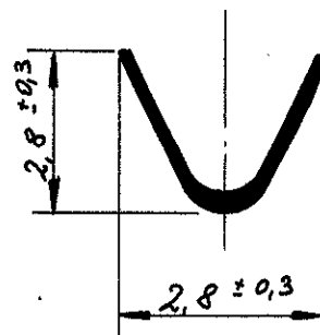
ISOL. PRESSHÜLSE
