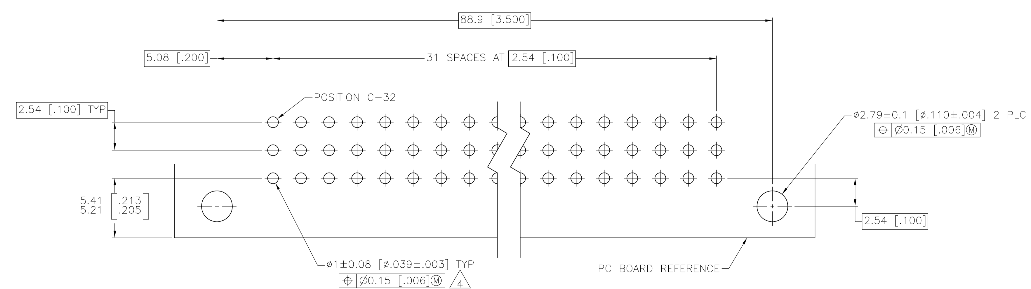
PC BOARD LAYOUT
