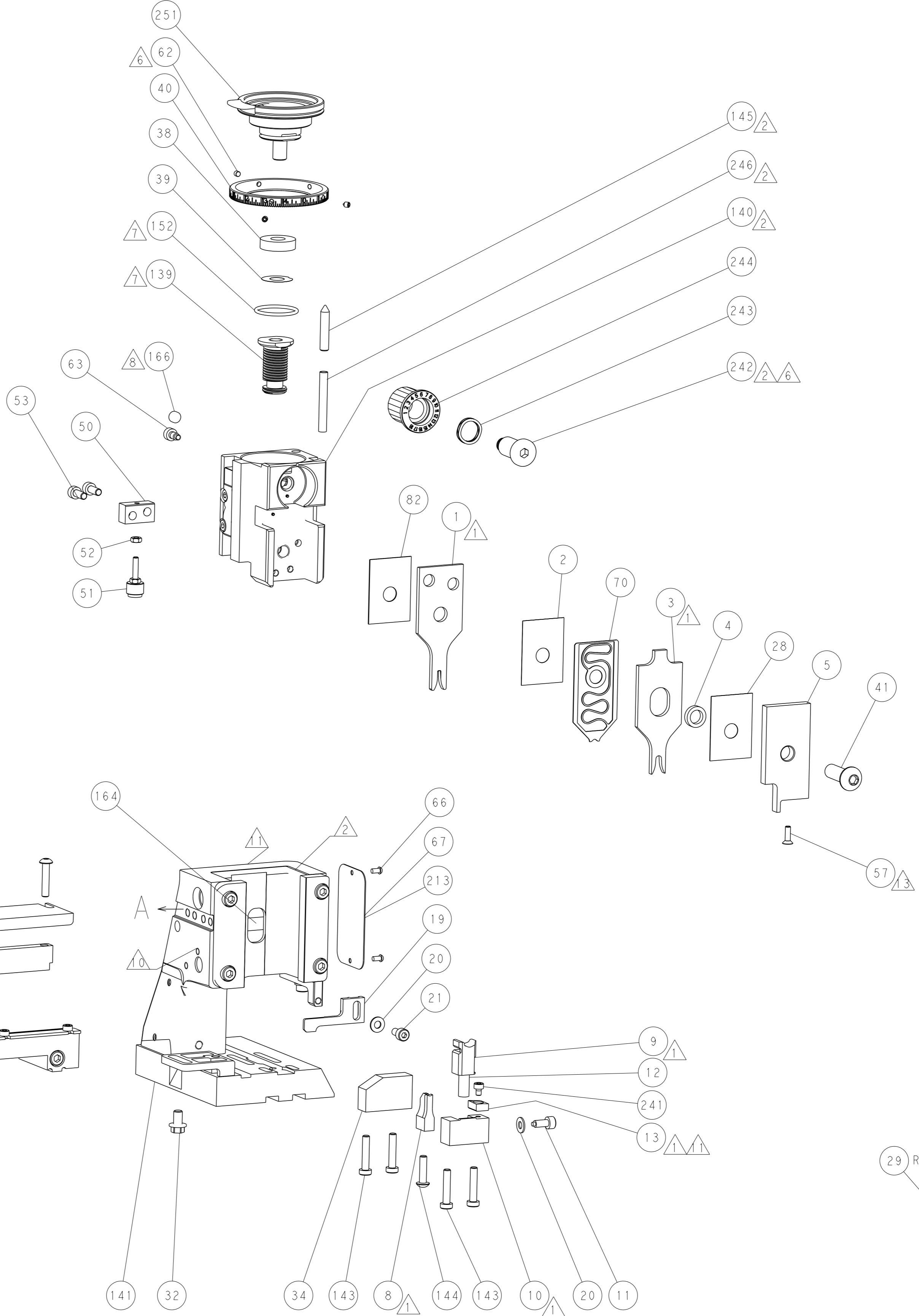
ITEM 30 LOCATED AT FRONT HOLES
